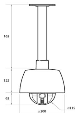
Ceiling Mount Bracket
